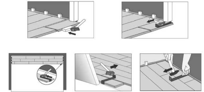
Fig 3: Use tapping block and pull bar to work under door frames and other obstacles.
